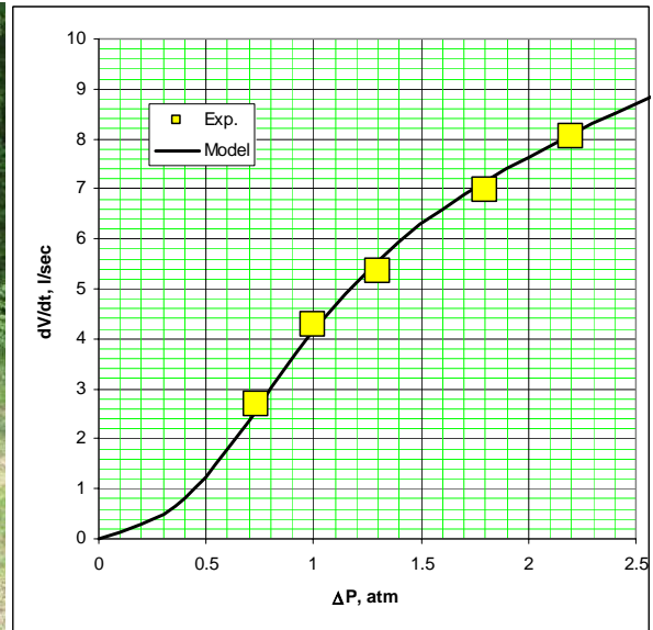
Methane leakage calibration
