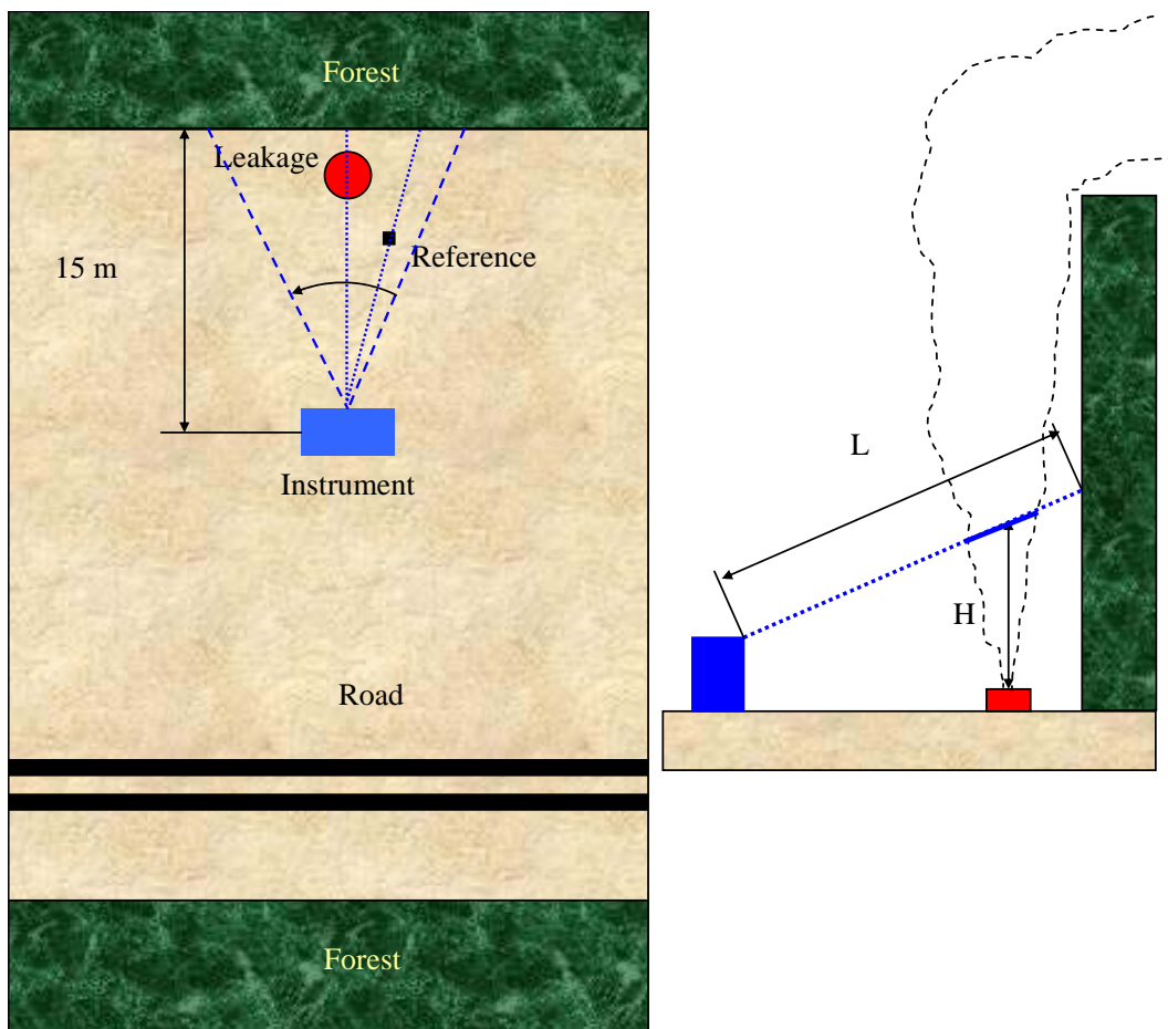
Scheme of experiment and view of instruments used
