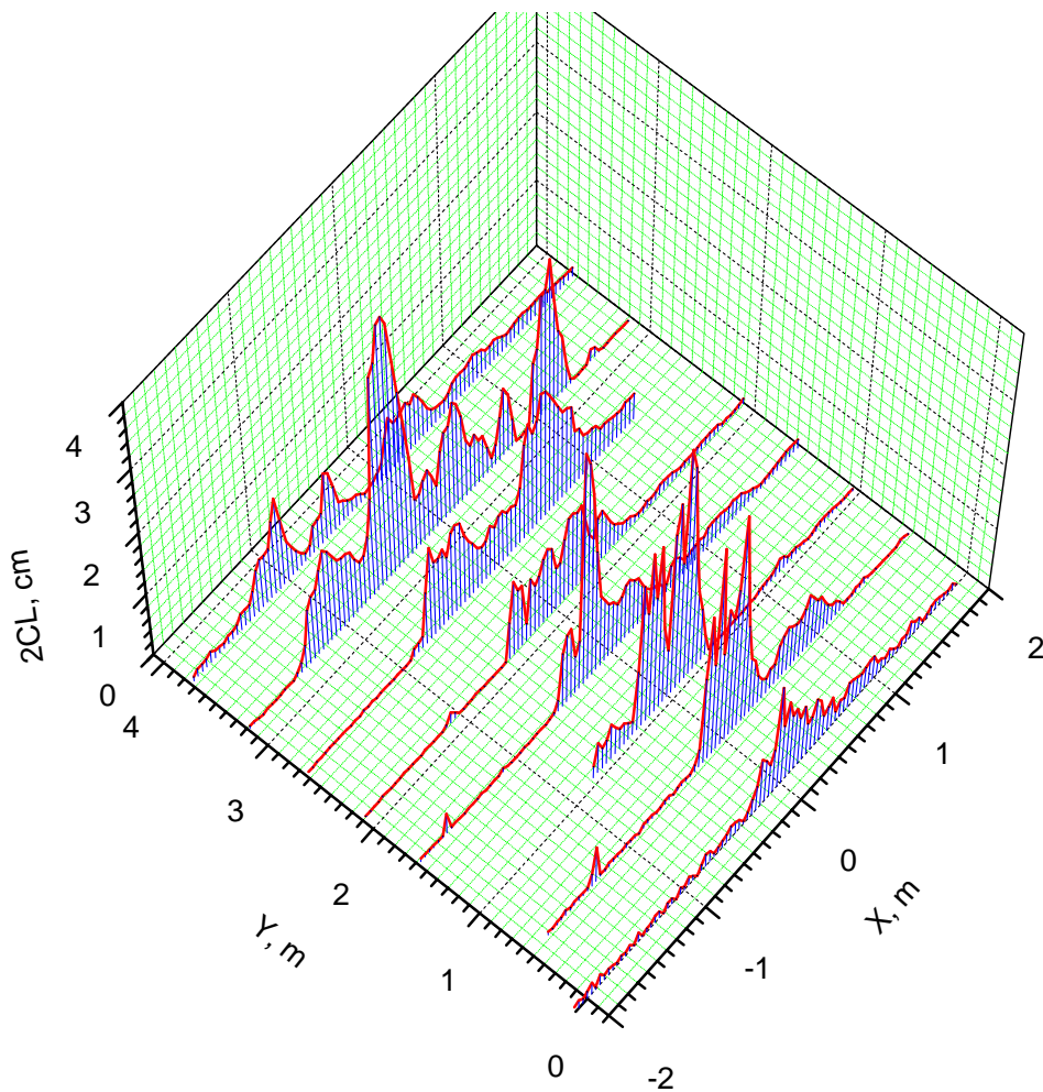
Cross sections of methane plume from calibrated leakage 1.2 l/sec
